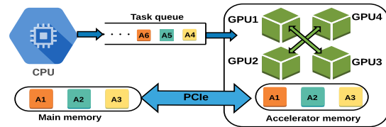
Figure 1: Application queue on a node with multiple GPUs.
